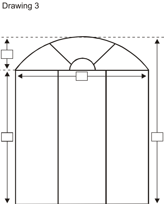
Measurements required for inside mount for arched headrails with floor length vanes.
