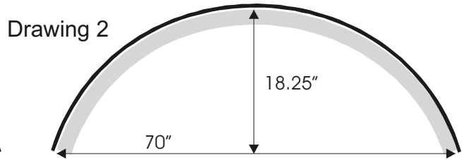
Headrail measurement
