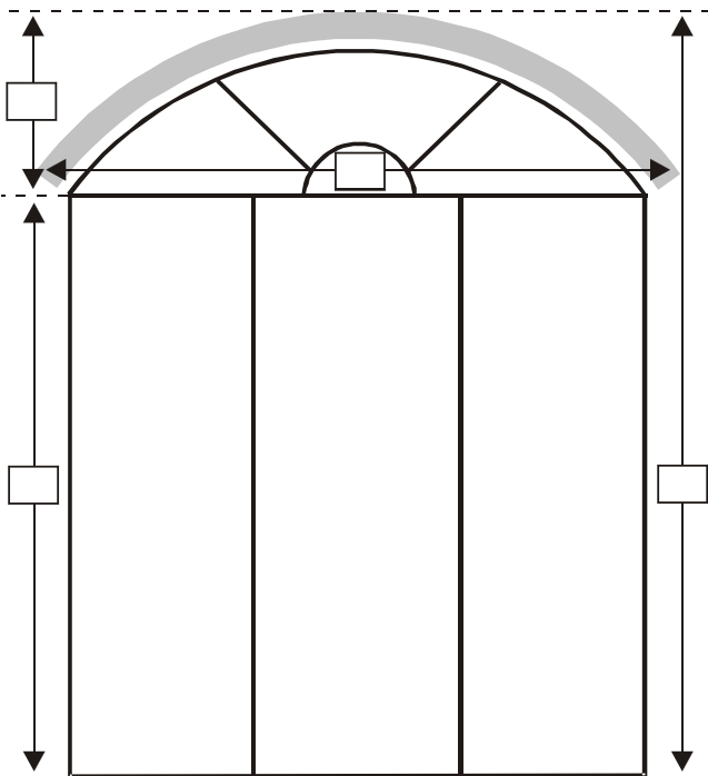
Measurements required for outside mount for arched headrails with floor length vanes.
